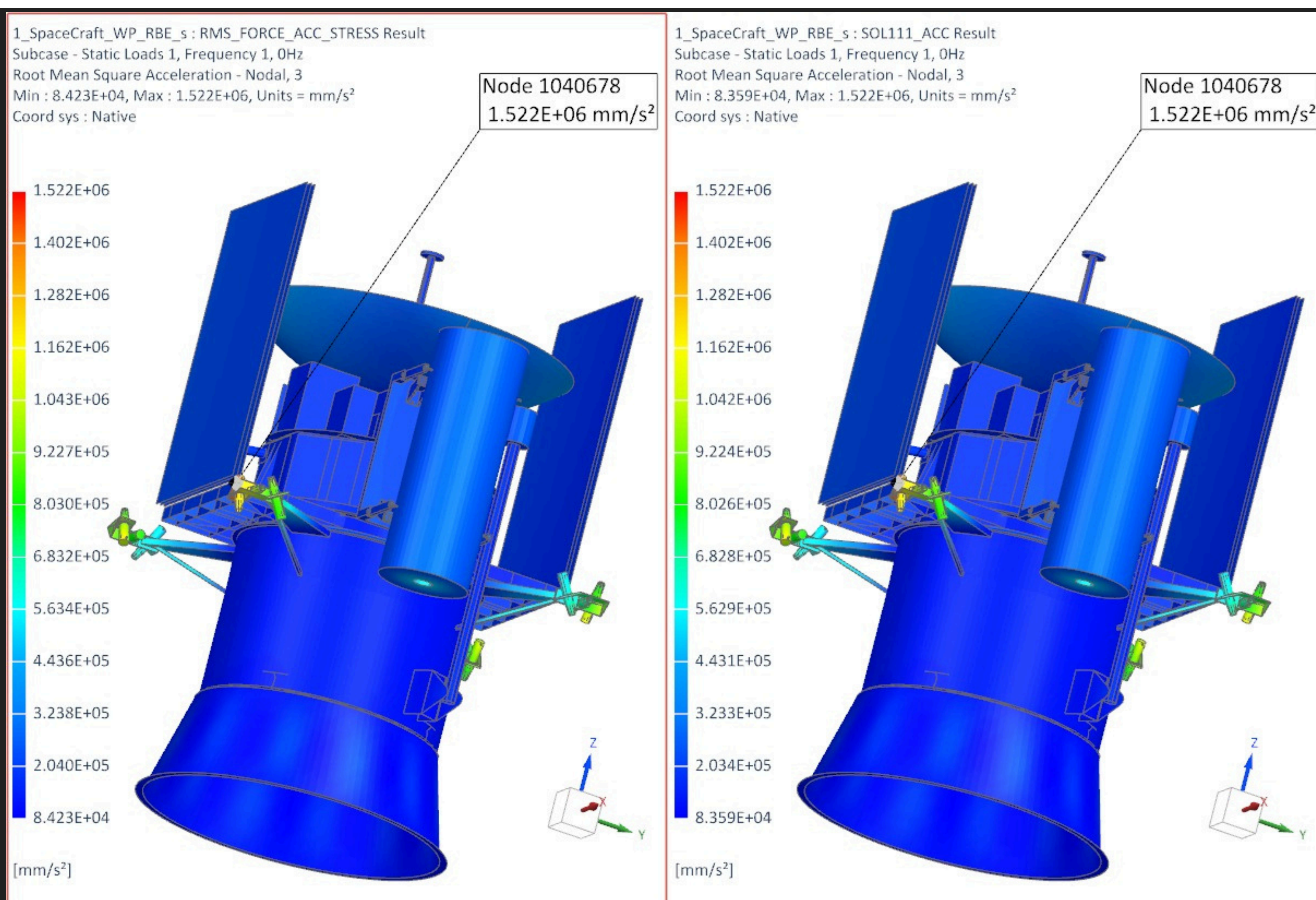
Figure 8: RMS Z-Acceleration Contours
