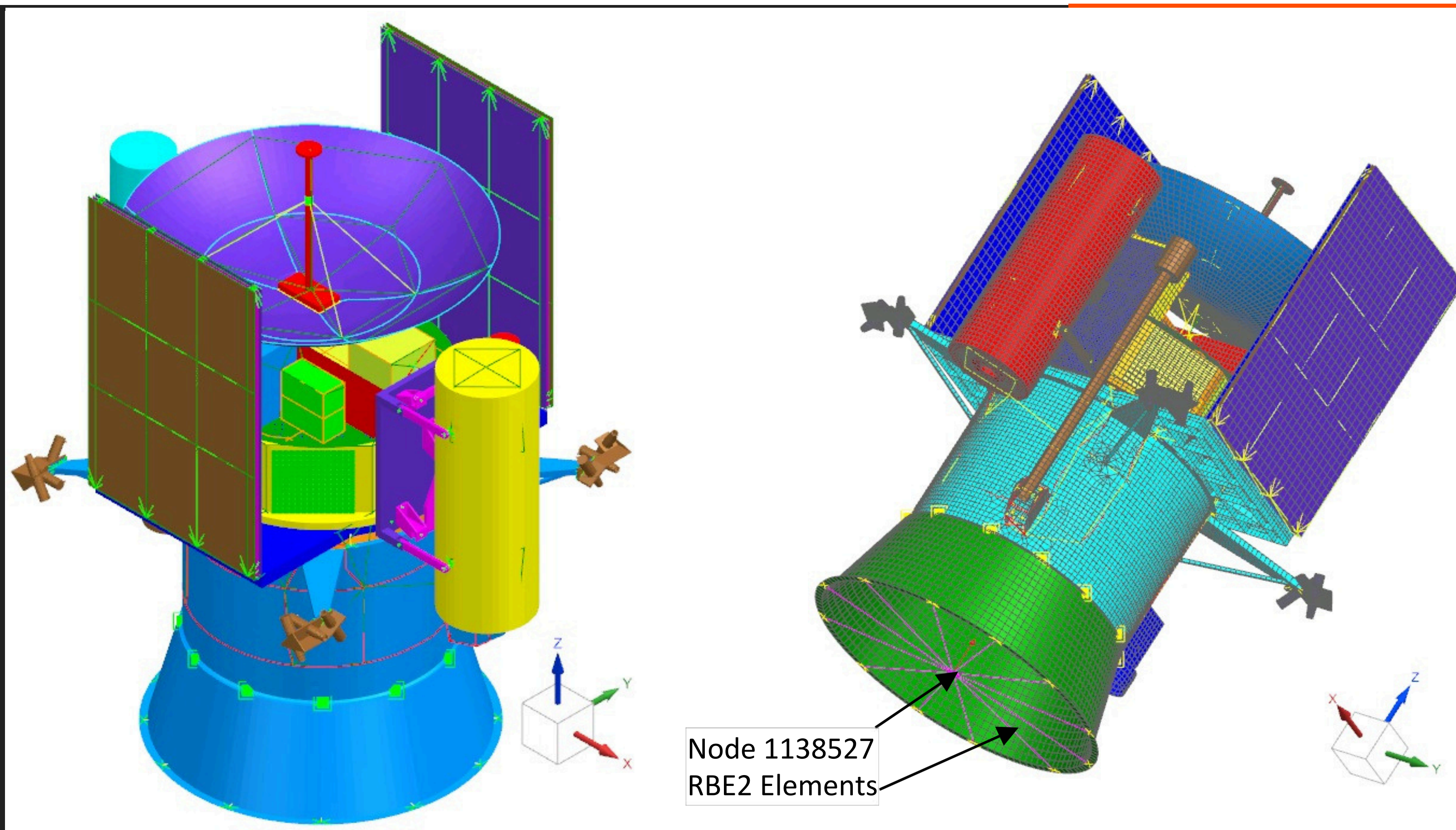
Figure 6: Spacecraft model, base acceleration was applied at node 1138527.
