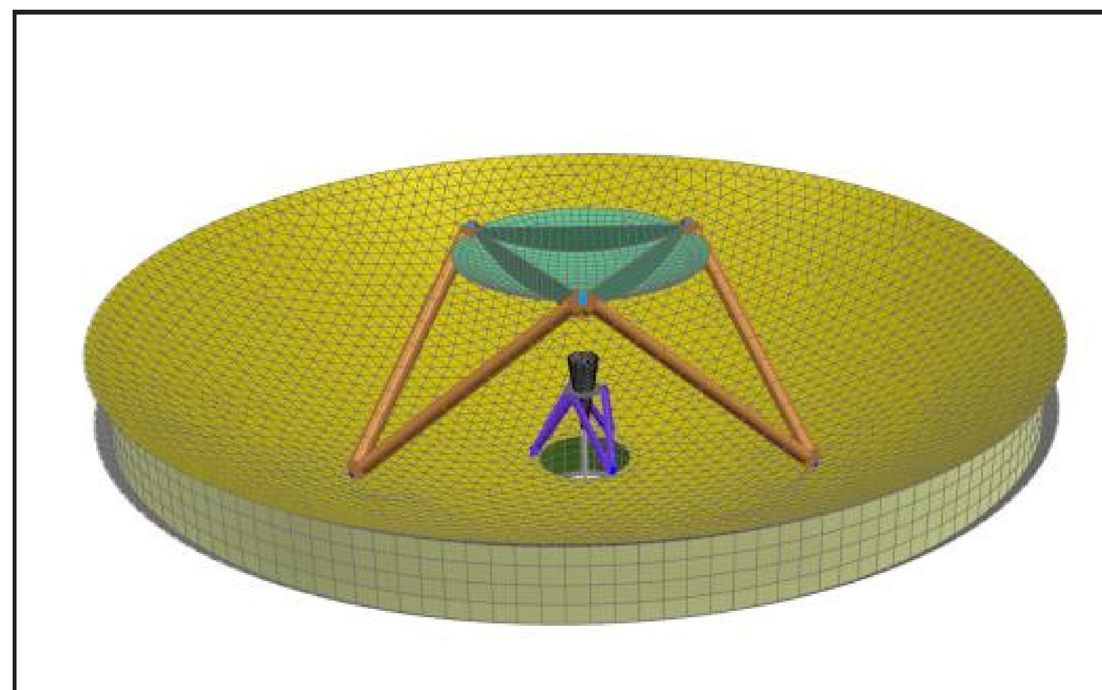
Figure 5 Space Antenna Model
