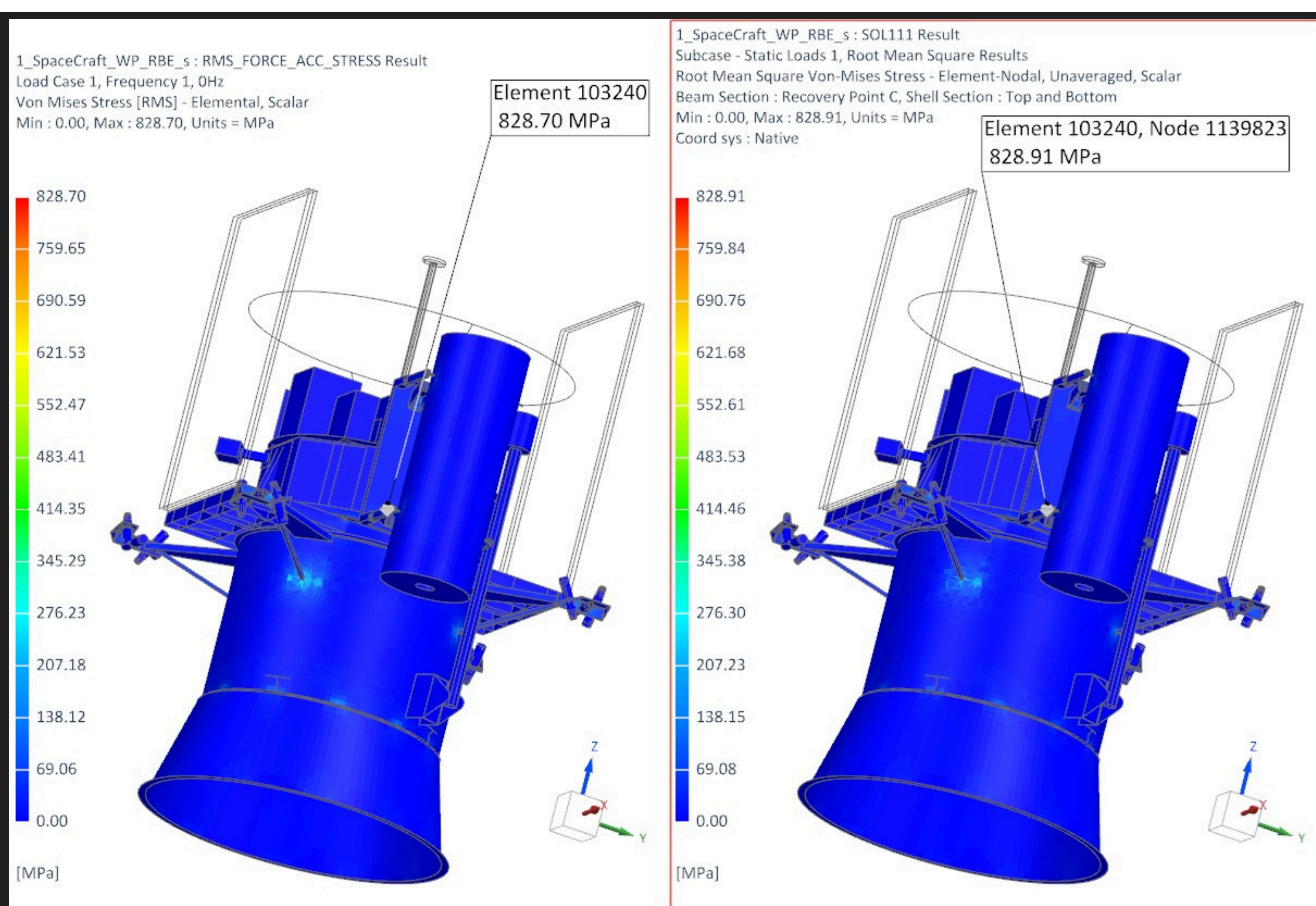
Figure 11: RMS Von Mises Stress Contours
