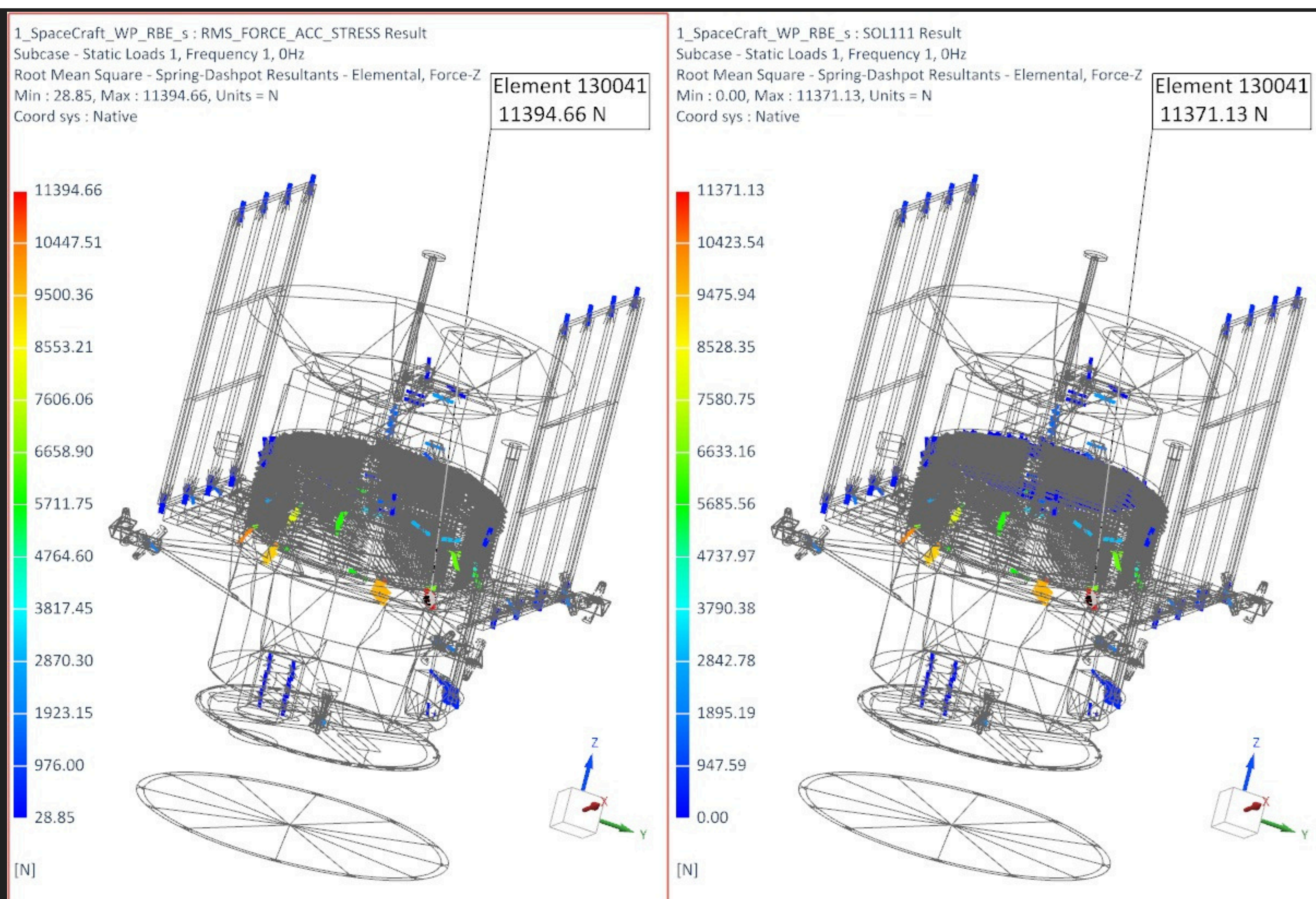
Figure 9 RMS Z-Force Contours
