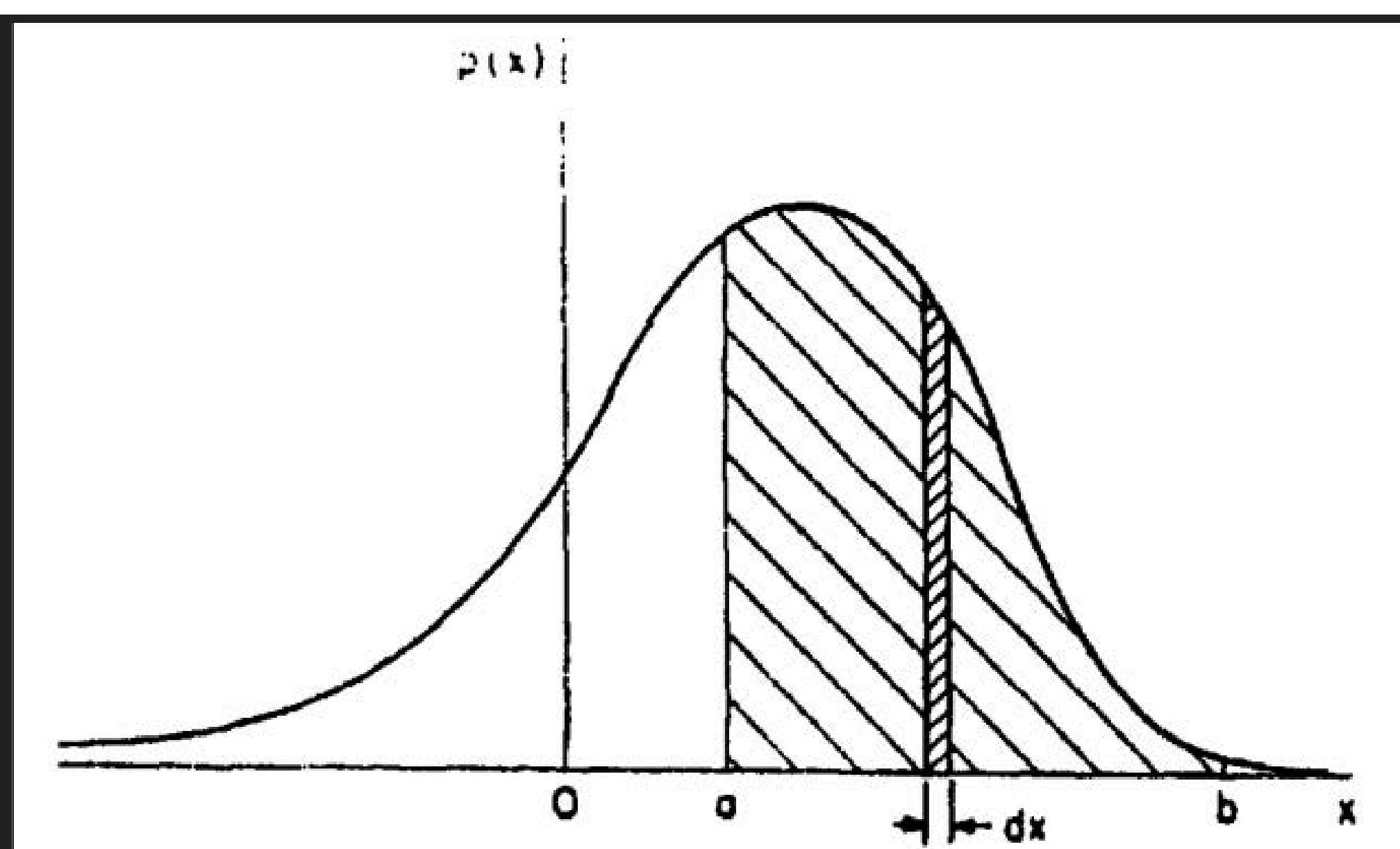
Figure 2: Probability Density Function of parameter X
