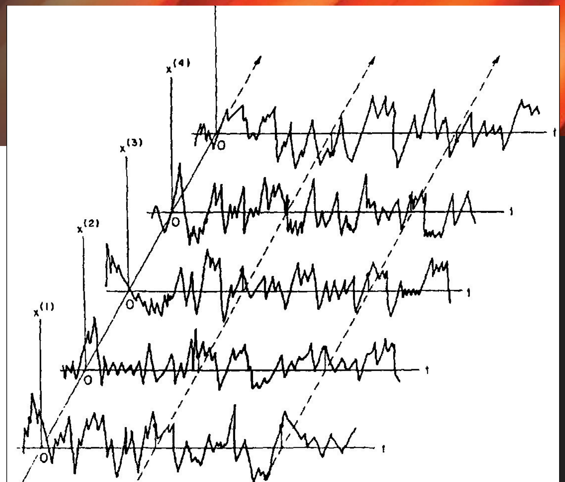
Figure 1: Random Process is Probabilistic, Not Deterministic.
