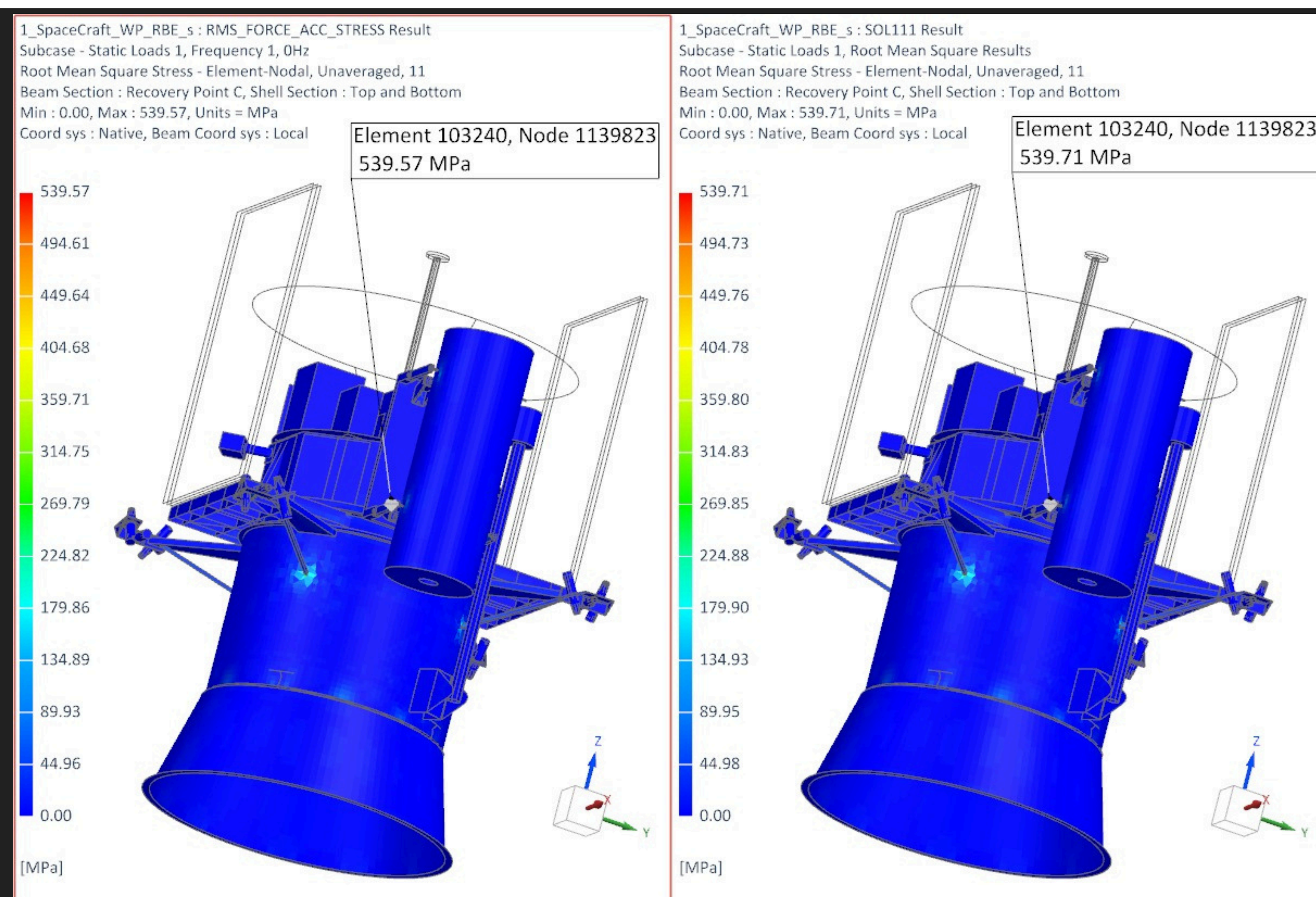
Figure 10 RMS XX Stress Contours
