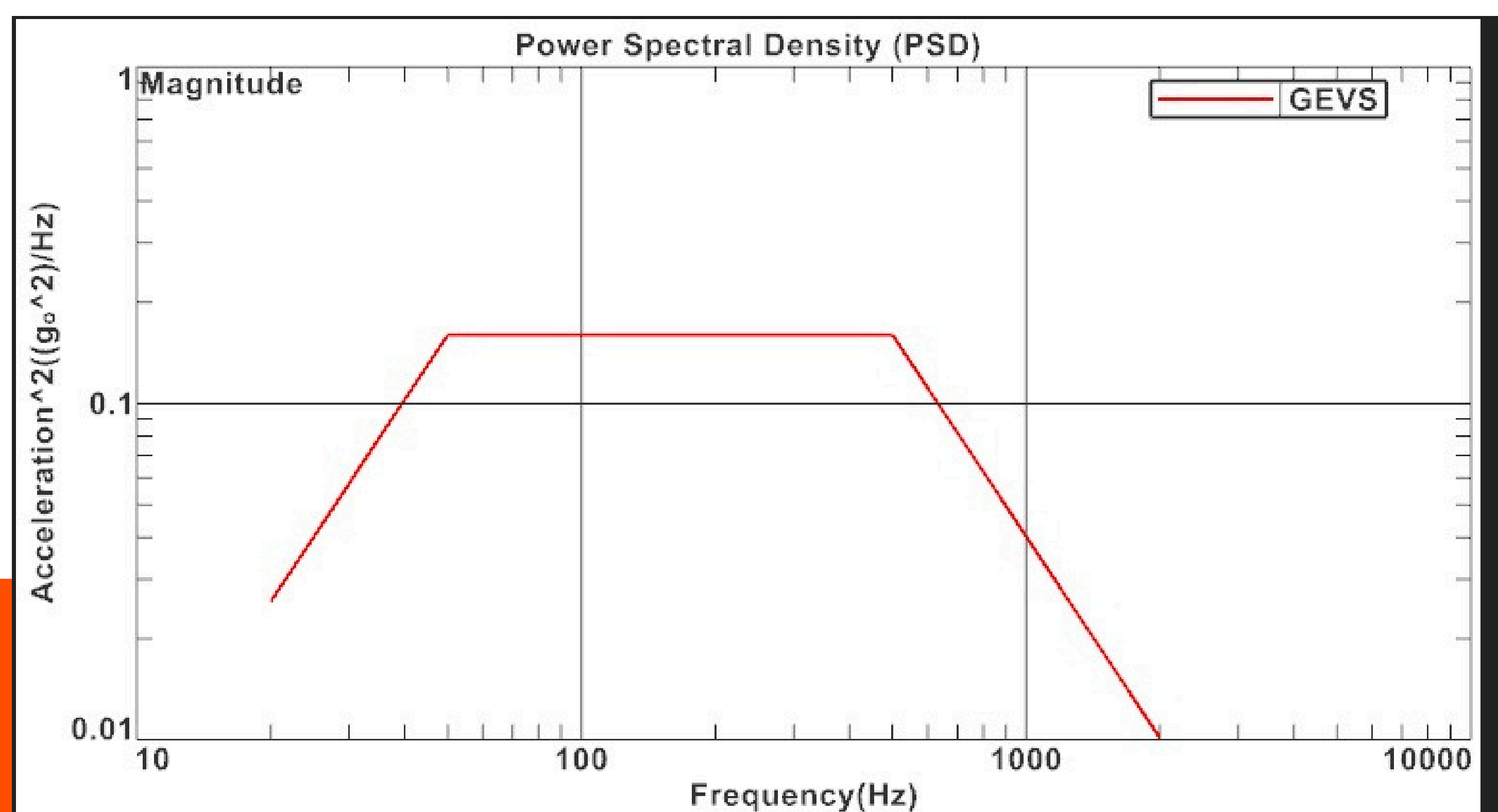
Figure 7: PSD input for base acceleration.
