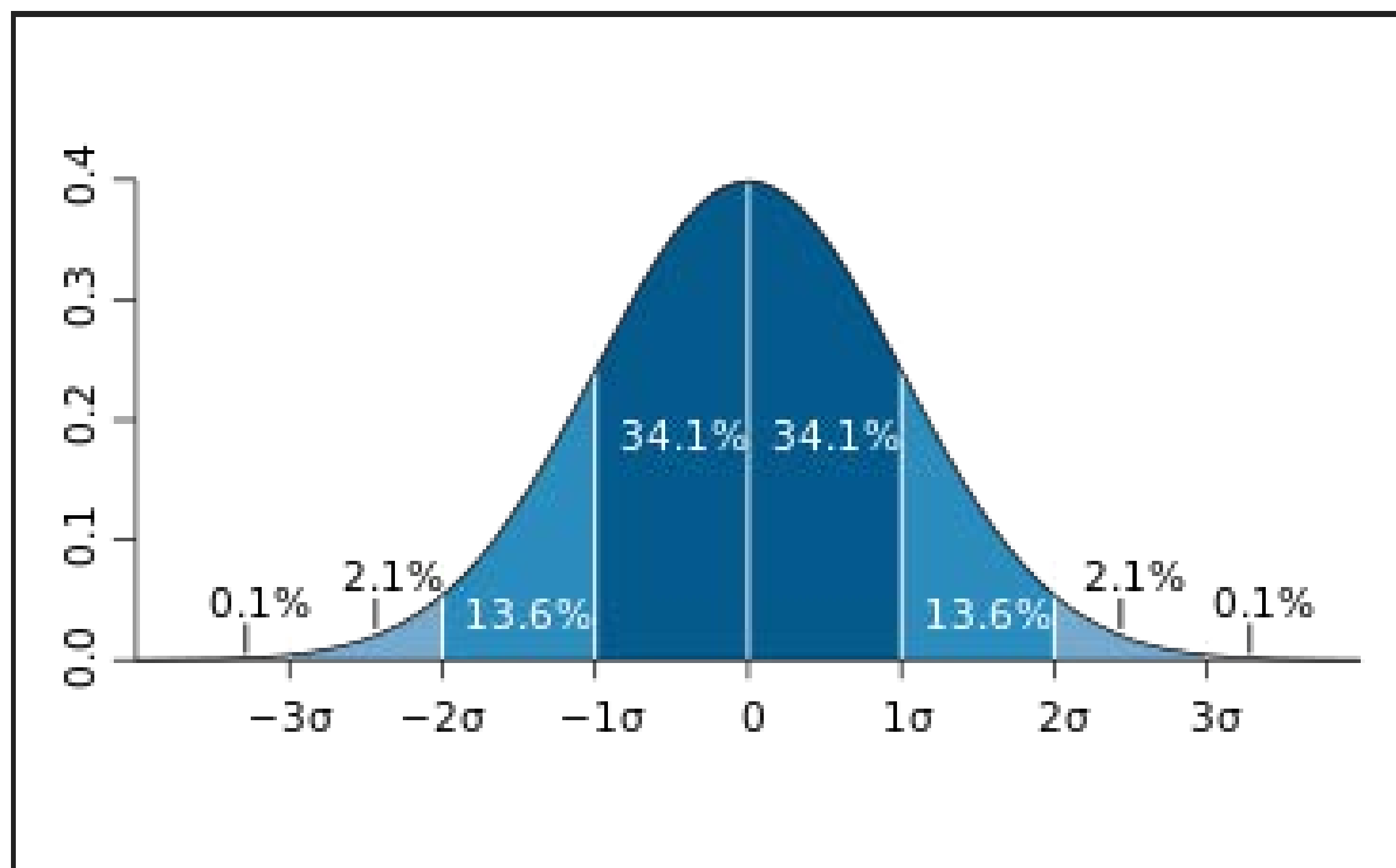
Figure 3: Normal (Gaussian) distribution curve, showing the probability as a function of standard deviation [Source: Wikipedia].
