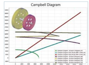
Rotor dynamics
